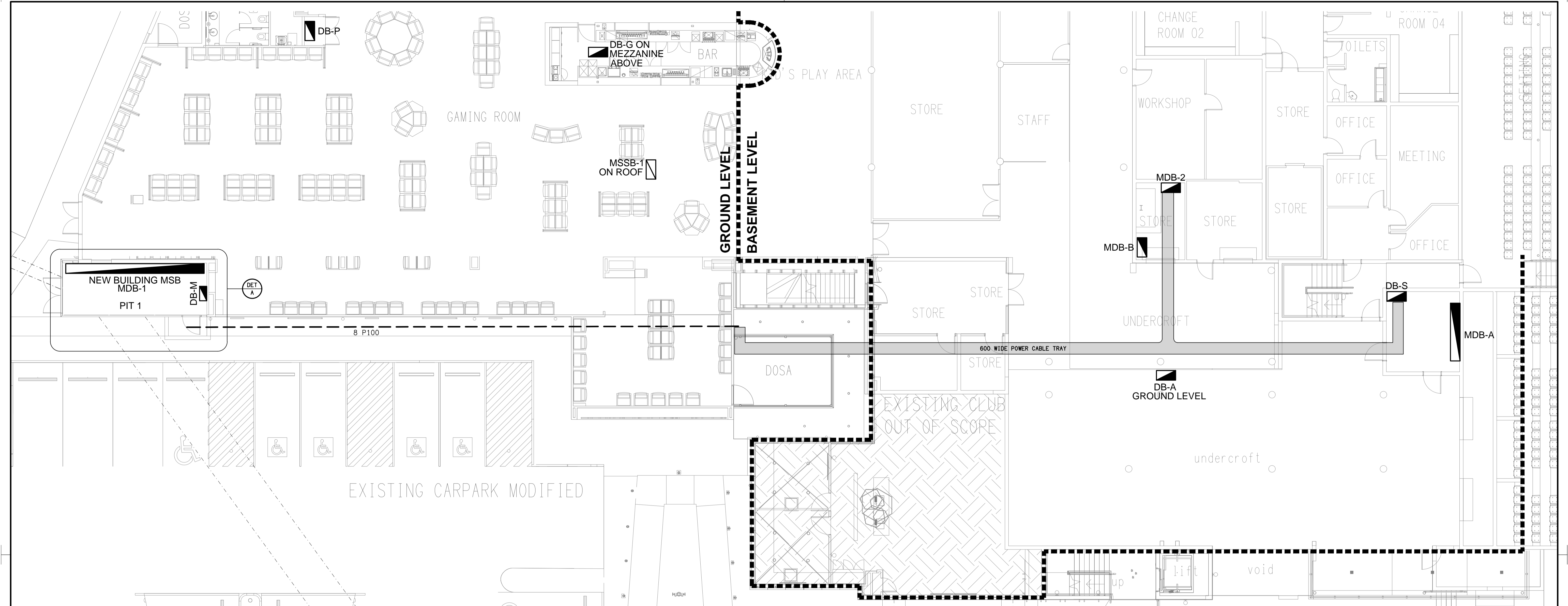
FLOOR PLAN CABLE ROUTE LAYOUT SCALE 1:100
