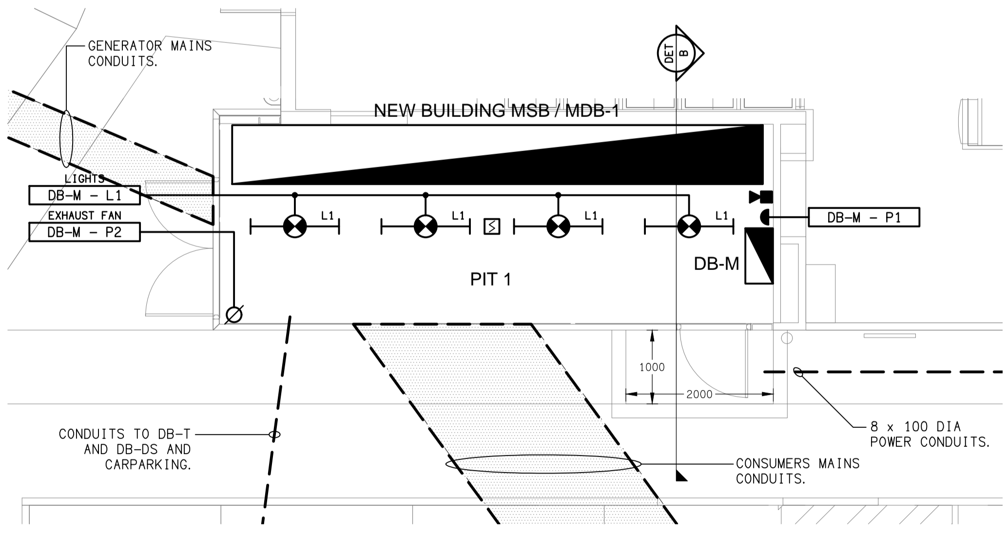
DETAIL A MDB-1 ROOM PLAN VIEW SCALE 1:50
